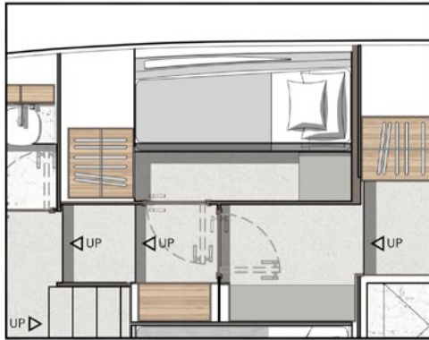
LOWER DECK OPTION Shown with stbd Pullman cabin
